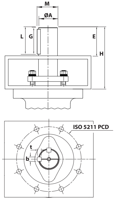
Trunnion Trim 60-105 Floating ball valve - Trim 60, 68
